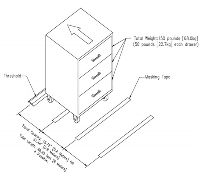
Figure 4. Rolling Stability Test Configuration
