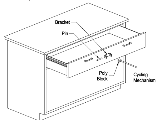
Figure 11. Drawer Cycling Mechanism Test Configuration
