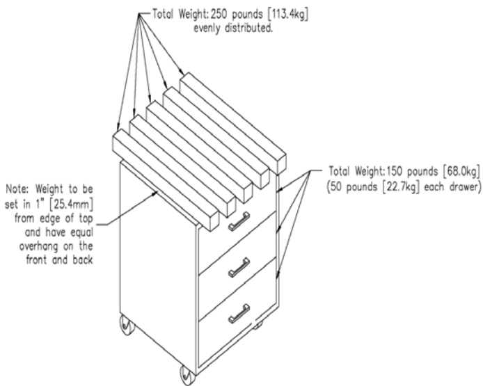
Figure 3. Static Load Test Configuration
